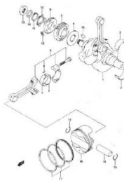
FIG.7 CRANKSHAFT (C-3)
