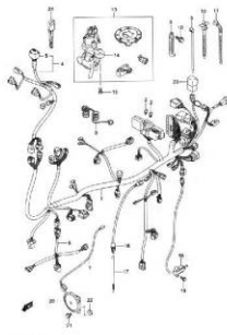
FIG.33 WIRING HARNESS (MODEL K2) (G-11)
