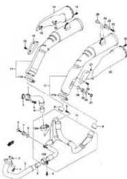
FIG. 14 MUFFLER (D-3)
