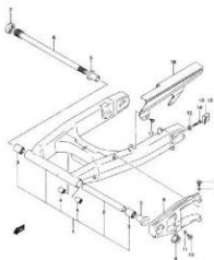
FIG.61 REAR SWINGING ARM (K-2)
