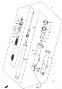
FIG.54A FRONT DAMPER (MODEL K3/K4) (I-7)
