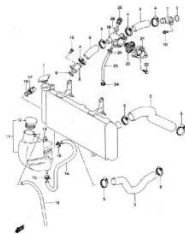
FIG.20 RADIATOR HOSE (D-11)
