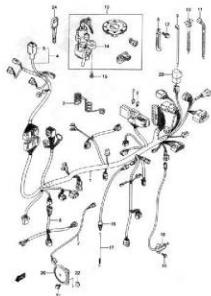
FIG.35 FRAME (H-2)
