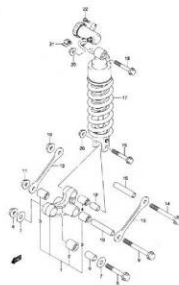
FIG.62 REAR CUSHION LEVER (K-3)
