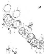
FIG.29 SPEEDOMETER (MODEL K2/K3) (G-2)
