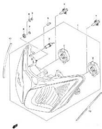
FIG.30 HEADLAMP (G-4)
