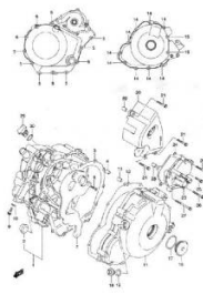
FIG.6 CRANKCASE COVER (C-2)
