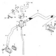
FIG.21 2ND AIR (D-12)
