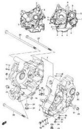
FIG.5 CRANKCASE (B-6)
