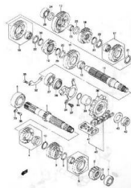
FIG.23 TRANSMISSION (MODEL K2/K3) (E-4)
