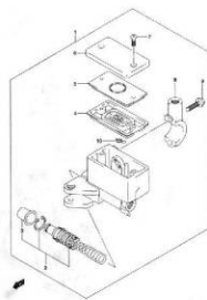
FIG.59 FRONT MASTER CYLINDER (J-12)
