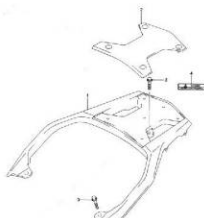
FIG.38 CARRIER (H-5)
